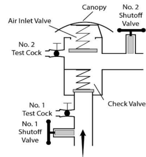
Direction of Flow Pressure vacuum breaker back-siphonage prevention assembly ZURN WILKINS 720A
