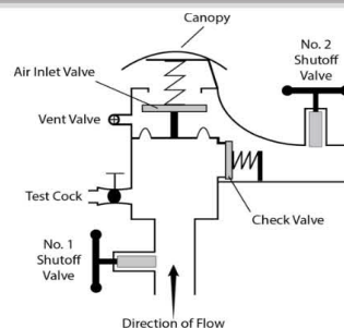
Spill-resistant pressure vacuum breaker backsiphonage prevention assembly ZURN WILKINS 460XL
