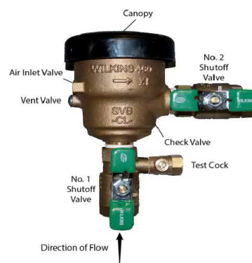
Spill-resistant pressure vacuum breaker backsiphonage prevention assembly ZURN WILKINS 460XL
