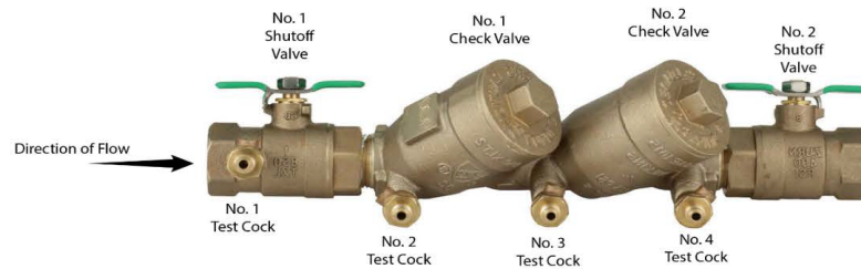
Double check valve backflow prevention assembly ZURN WILKINS 950XLT2
