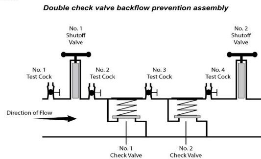
Double check valve backflow prevention assembly ZURN WILKINS 950XLT2
