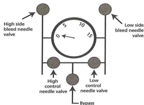
Five Valve
