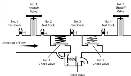
Reduced pressure principle backflow prevention assembly ZURN WILKINS 775XL3
